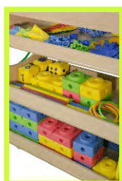
No 171703 4-storeyed Psychomotor Objects Storage Trolley Made of solid baked beech wood with reinforced caster wheels with brake. It has special spots for rhythmic gymnastics and psychomotor objects placement. Dimensions: 98 x 69 x 107 cm
